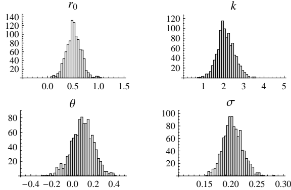
Figure 2: Learned parameters 50 bins histograms.
